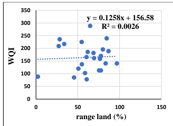
e. Relationship between range land (%) and WQI
